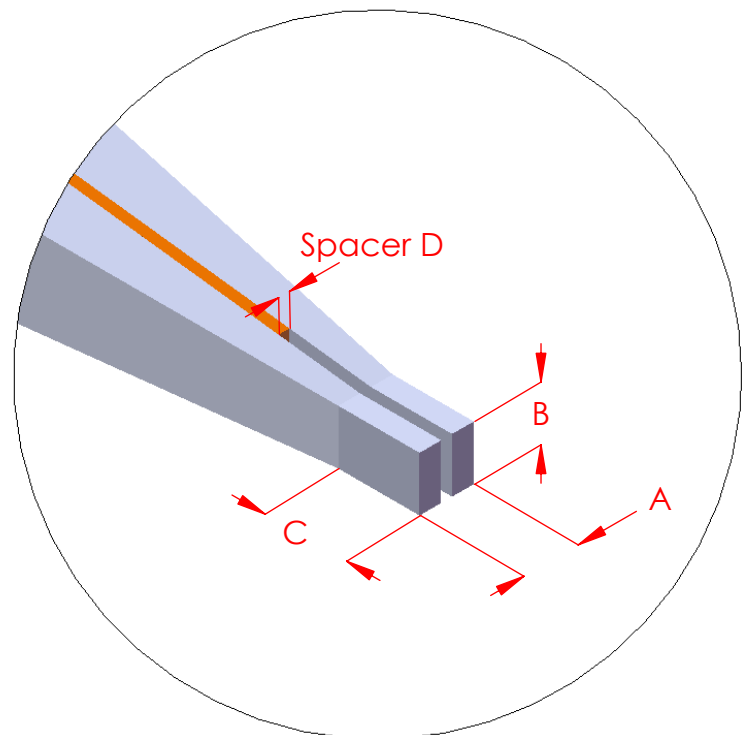
DETAIL VIEW F SCALE 40 : 1
